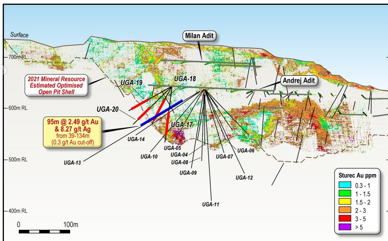
Figure 3: Long-section showing the traces of drill holes from the current drill program from Drill Chamber 2, as well as the previous Phase 1 drill program from Drill Chamber 1; shown relative to mineralisation within the existing Sturec Mineral Resource displayed as a 3D point cloud (grade scale shown with pseudocolor spectrum). This view is looking west
